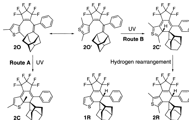
Scheme 3. Formation of by-product from 20 .
