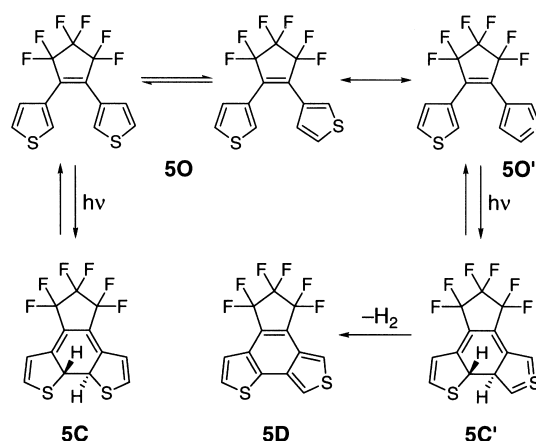
Scheme 2. Formation of by-product from 50 .
