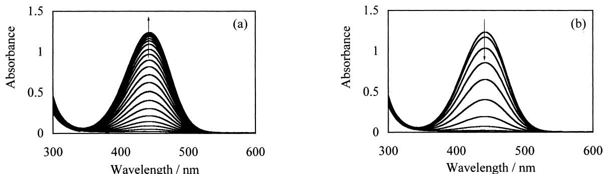
Fig. 2. Change in absorption spectra in toluene. (a) Irradiation of 313-nm light. Irradiation time/min; 0, 0.5, 1.5, 3, 5, 8, 12, 17, 23, 30, 38, 47, 57, 68, 80, 95, 110, 125, 140, 155, 170, 185, 200. (b) Irradiation of 405-nm light. Irradiation time/min; 0, 0.5, 1.5, 3, 5, 8, 12, 17, 23, 30, 38.
