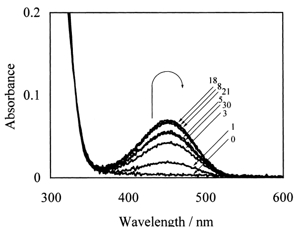
Fig. 1. Absorption spectral change of 2 during 313-nm light irradiation in toluene. Irradiation time/min; 0, 1, 3, 5, 8, 18 (largest absorbance at 450 nm), 21, 30.
