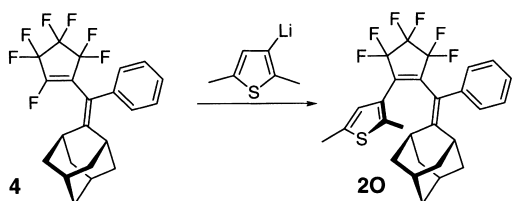
Scheme 1. Synthesis of 20 .
