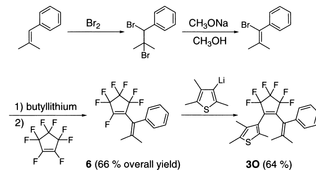
Scheme 4. Synthesis of 3O .
