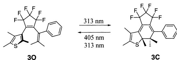
Scheme 5. Photoreaction of 30 .
